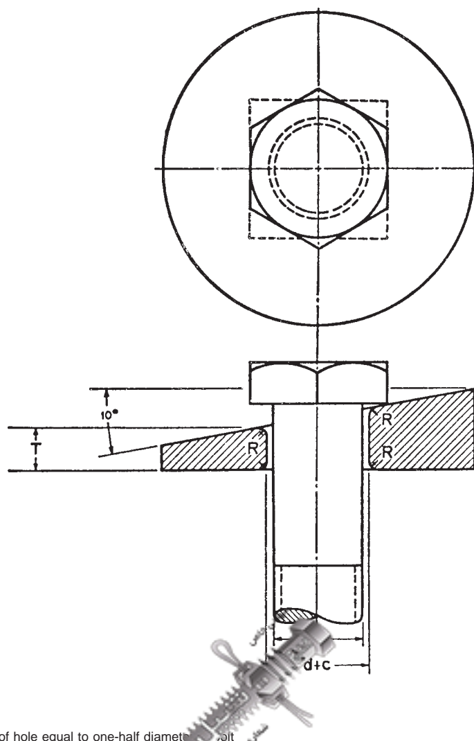
FIG. A3.2 Wedge Test Detail
